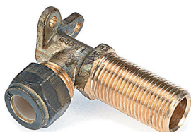
19BP MALE COMPRESSION ELBOW LUGGED (COPPER OLIVE)
